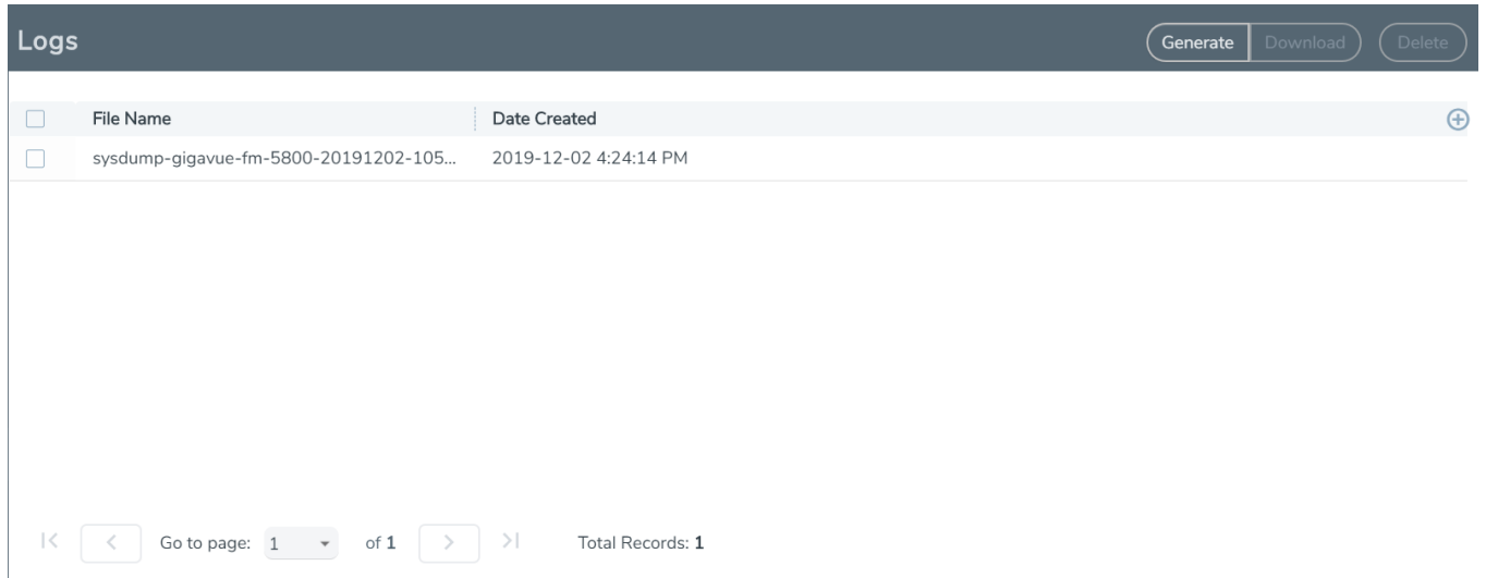
Figure 20 Logs Page
