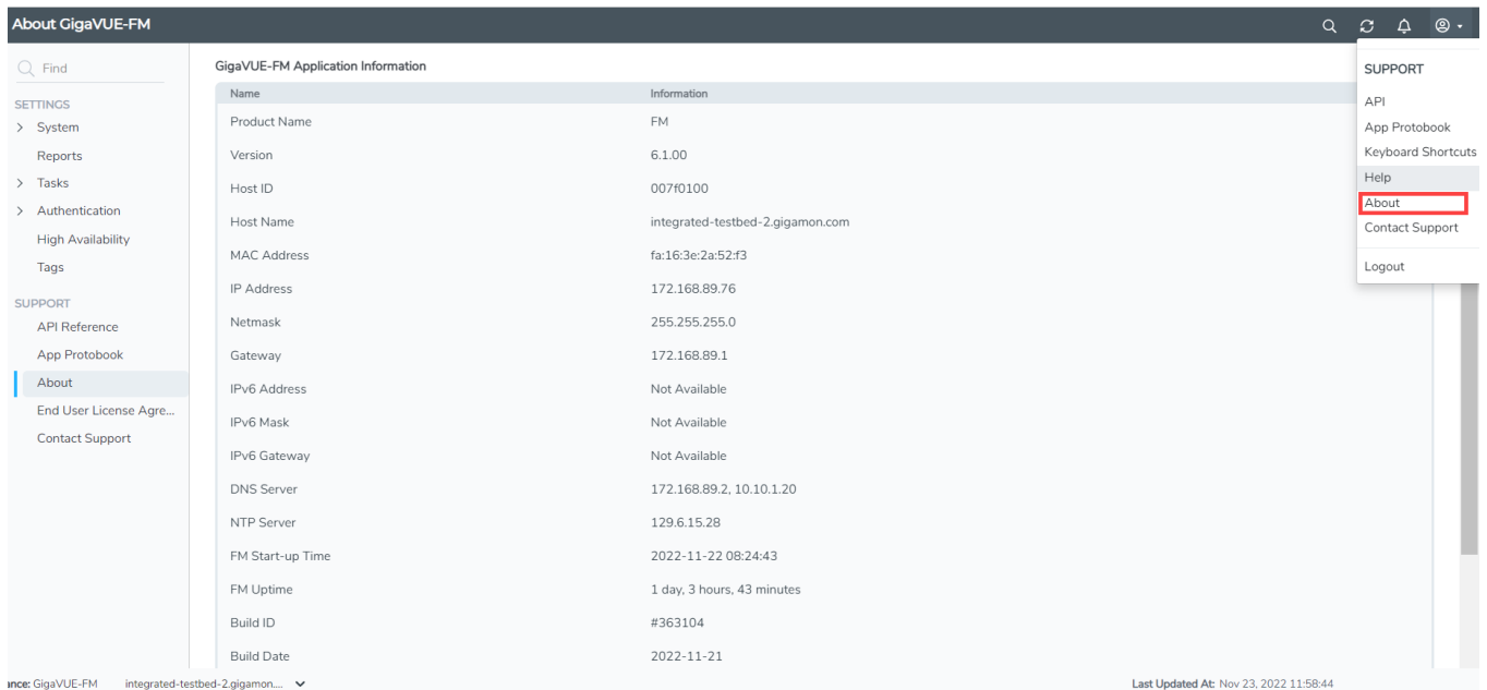
Figure 30 About Page
