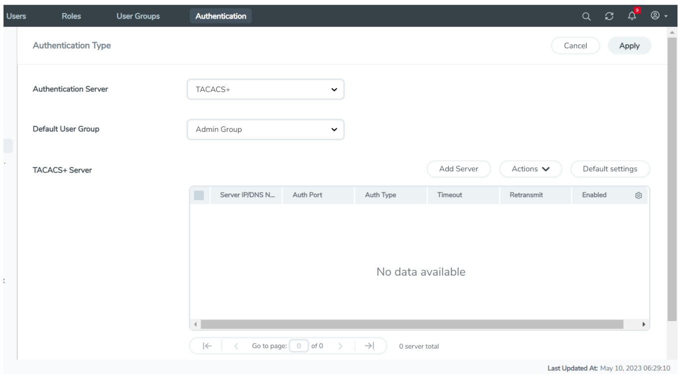
Figure 3 TACACS+ Page
